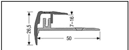
PF 320 Treppenkantenschiene 7-16 mm
